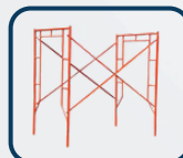
SCAFFOLD H-FRAME Size : 2.0M x 2.5M Finish : Painted/HDG
